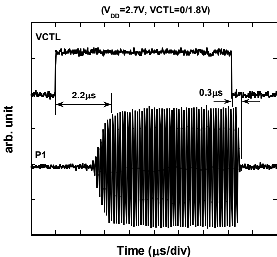
Switching Time
